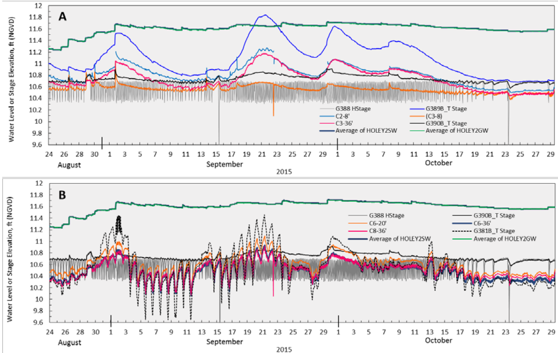
Figure 8. Hydrographs of surface water stages and groundwater elevations at 30-minute intervals for (A) the PSTA Cell, LSAV Cell, Holey Land WMA, and wells in the PSTA Cell's east levee, and (B) the PSTA Cell, STA-3/4 Discharge Canal, Holey Land WMA, and wells in the PSTA Cell's west levee from August 24 to October 29, 2015. (Note: HStage – headwater stage and TStage – tailwater stage.)
