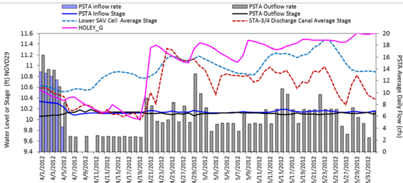
Figure 4. Daily average stages in the LSAV Cell, STA-3/4 Discharge Canal, and Holey Land WMA, and at the PSTA Cell inflow and outflow locations together with daily average PSTA Cell inflow and outflow rates from April 1 to June 2, 2012.
