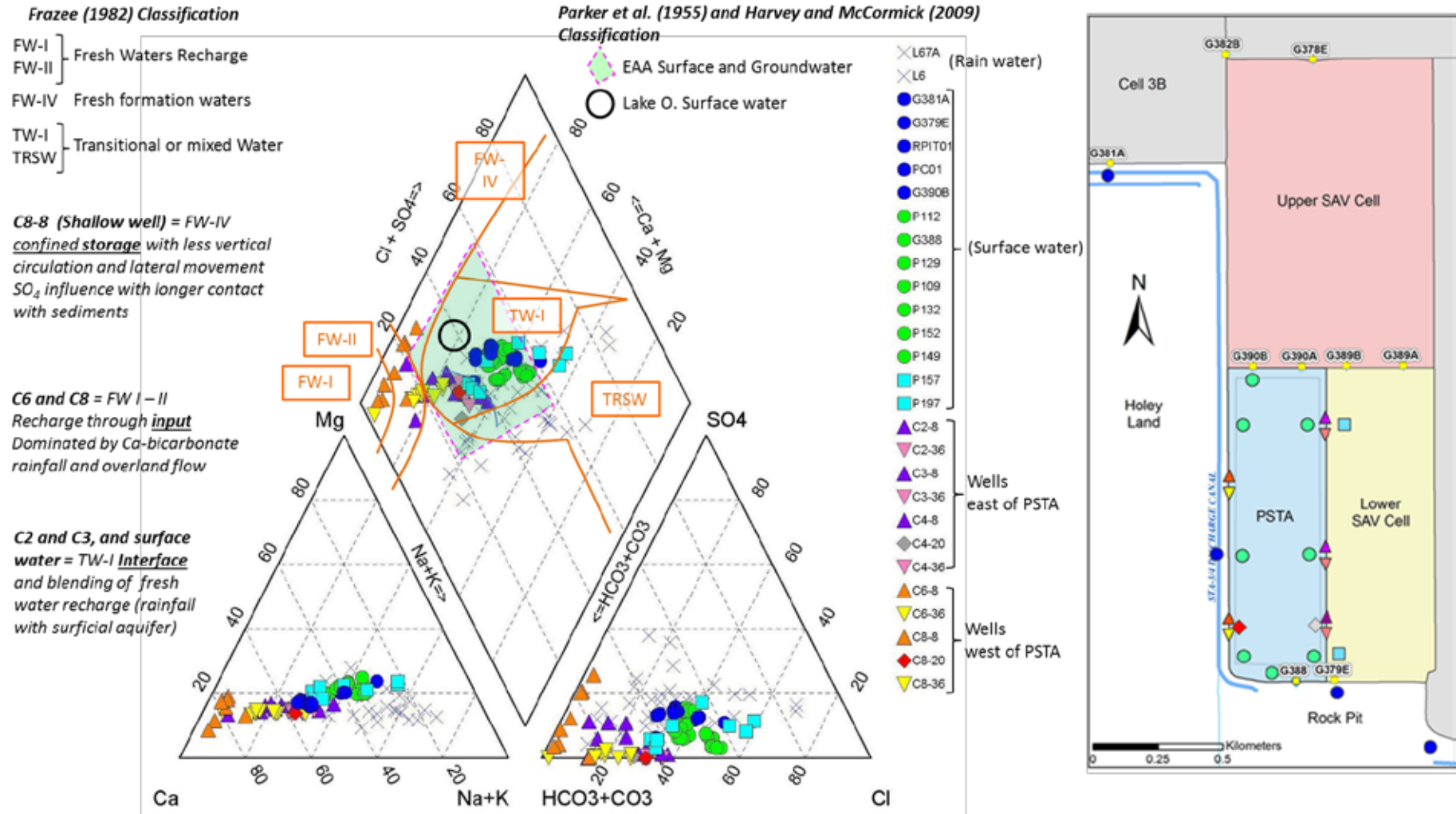
Figure 23. Piper diagram showing the chemical composition of rainwater, surface water, and groundwater collected from specific locations in the vicinity of the PSTA Cell indicating the areas of freshwater recharge (FW-I and FW-II), transitional or mixed water (TW-I) and freshwater confinement (FW-IV).
