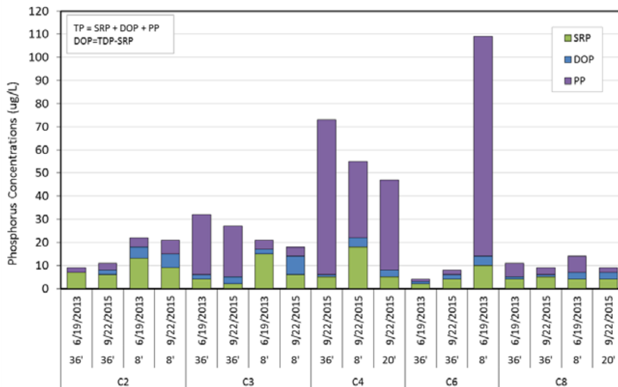
Figure 21. TDP and PP concentrations in groundwater samples collected from the shallow (8-ft) and deep (36-ft) PSTA Cell's levee wells. C2, C3, and C4, are in the east levee between the LSAV and PSTA cells; C6 and C8 are in the west levee between the PSTA Cell and STA-3/4 Discharge Canal.
