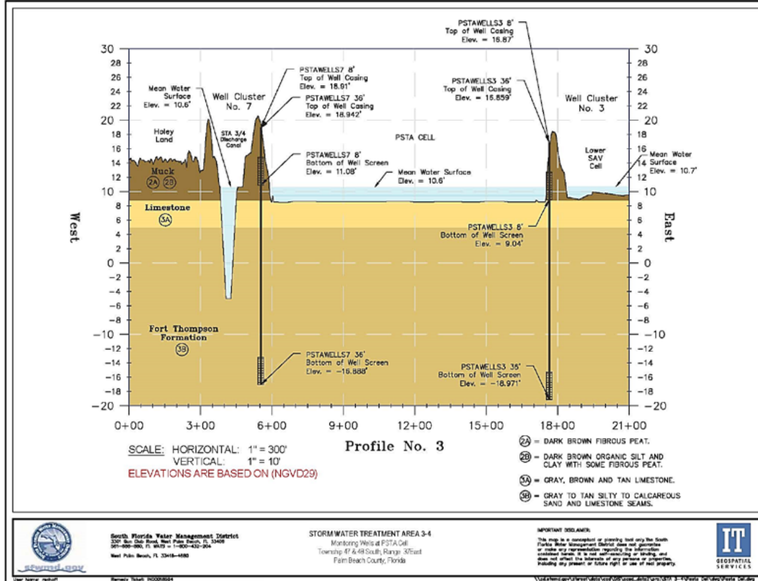
Figure A-4. West to east hydrogeologic cross-section profile through monitor well clusters C7 and C3 illustrating surficial aquifer formations underlying the Holey Land WMA, STA-3/4 Discharge Canal, PSTA Cell, and LSAV Cell.
