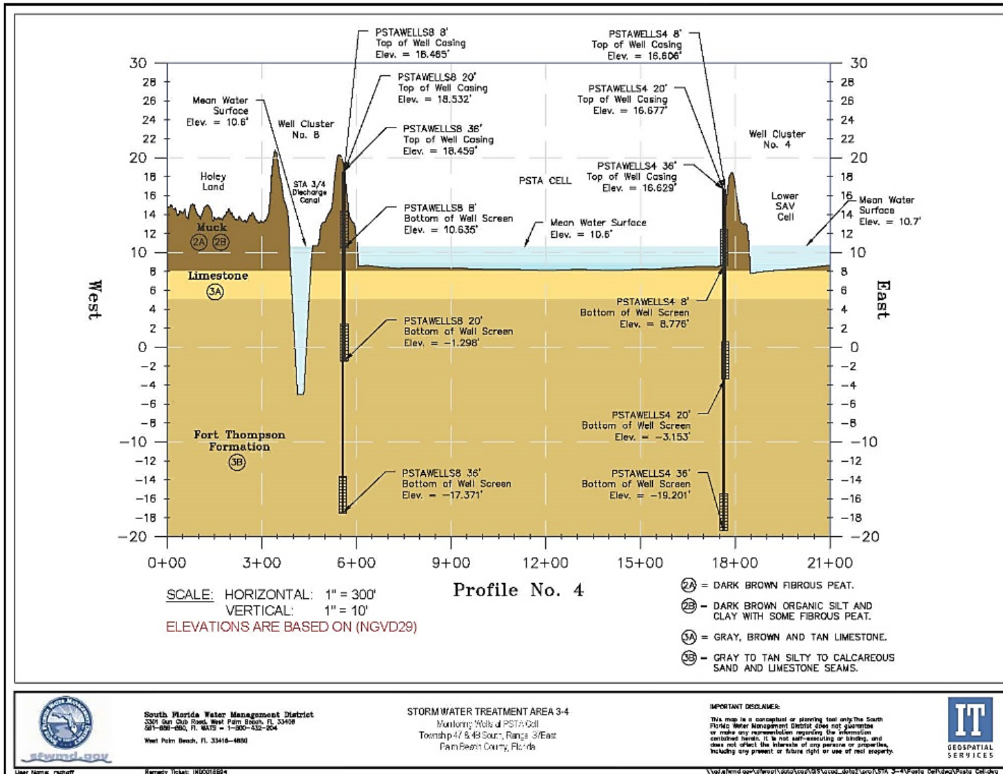
Figure A-5. West to east hydrogeologic cross-section profile through monitor well clusters C8 and C4 illustrating surficial aquifer formations underlying the Holey Land WMA, STA-3/4 Discharge Canal, PSTA Cell, and LSAV Cell.
