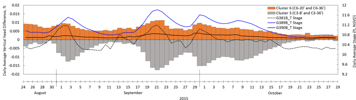
Figure 10. Daily average head differences in well clusters C3 (east levee) and C6 (west levee) in relation to the TW stage (T Stage) at G-389B (inflow to the LSAV Cell), TW stage at G-390B (inflow to the PSTA Cell), and TW stage at G-381B (outflow from STA-3/4 Cell 3B) into the STA-3/4 Discharge Canal. Positive and negative head differences indicate upward or downward hydraulic gradients, respectively.
