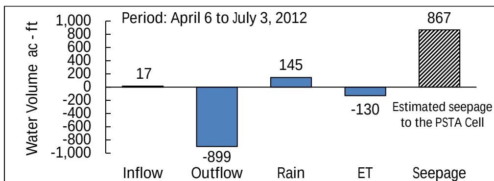
Figure 3. Water budget estimates for the PSTA cell, including total volume of inflow, outflow, rainfall, ET and seepage from April 6 to July 3, 2012.
