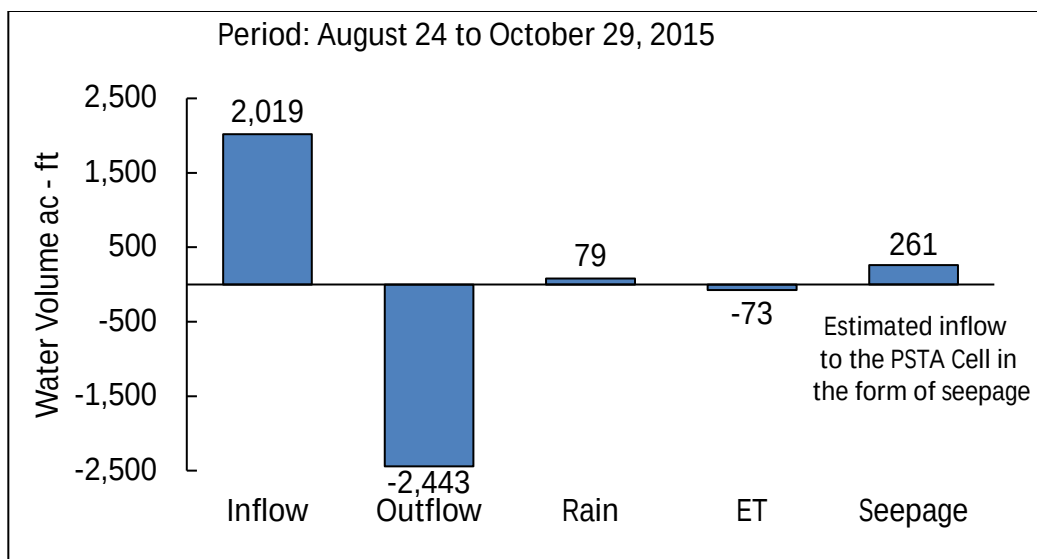
Figure 9. Water budget estimates for the PSTA Cell, including total volume of inflow, outflow, rainfall, ET, and seepage from August 24 to October 29, 2015.
