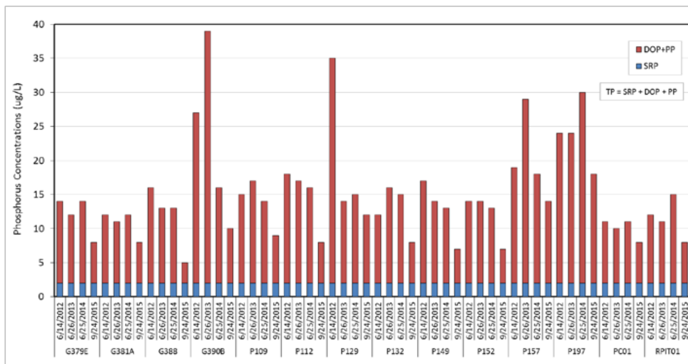
Figure 18. TP and SRP concentrations in surface water samples collected from sites within the PSTA Cell, LSAV Cell, and STA-3/4 Discharge Canal. (Note: µg/L – micrograms per liter.)
