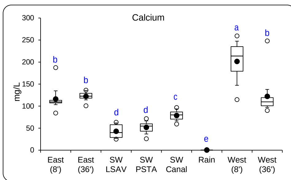
Figure 15. Comparison of Ca concentrations in rainwater, surface water in the LSAV and PSTA cells, and groundwater from shallow (8-ft) and deep (36-ft) wells along the PSTA Cell's east and west levees.
