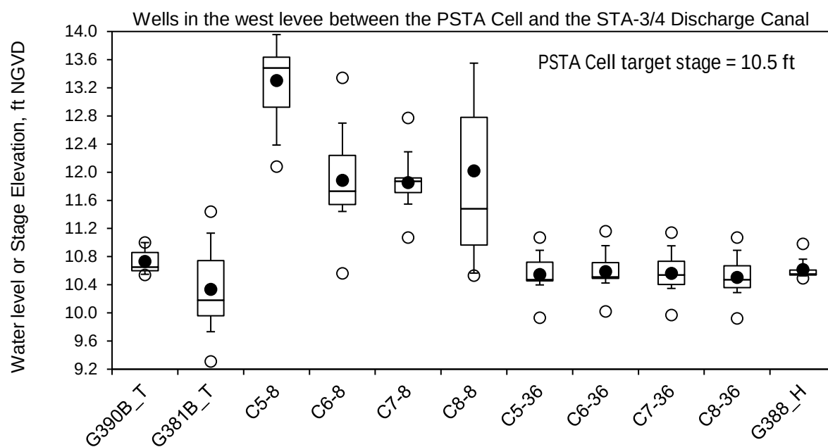
Figure 7. Comparison of groundwater elevations in the shallow (8-ft) and deep (36-ft) wells located in the levee between the STA-3/4 Discharge Canal and PSTA Cell prior to (A) and after (B) increasing the target stage. See Figure 6 for a description of the box plots.
