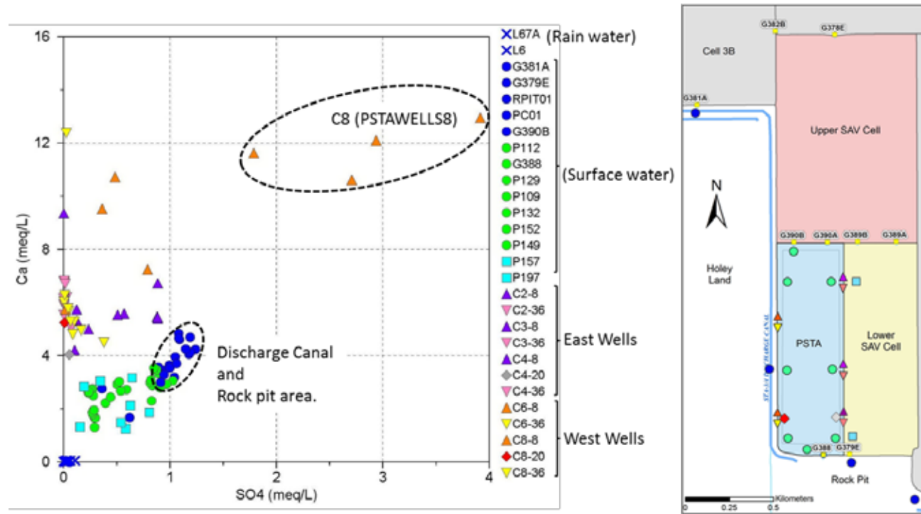
Figure 17. Scatterplot of Ca and SO 4 concentrations in water quality samples collected from surface water in the PSTA Cell, groundwater in the shallow (8-ft) and deep wells (36-ft) along the PSTA Cell's east and west levees, and rainwater at stations L67A and L6 (see Figure 2 ).
