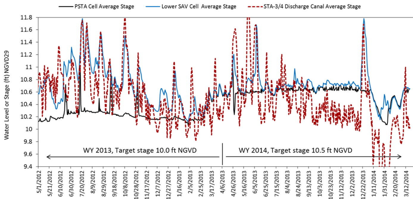
Figure 5. Daily average stages in the LSAV Cell, STA-3/4 Discharge Canal, and PSTA Cell during WY2013 and WY2014, before and after the target stage increase from 10.0 ft NGVD29 to 10.5 ft NGVD29.
