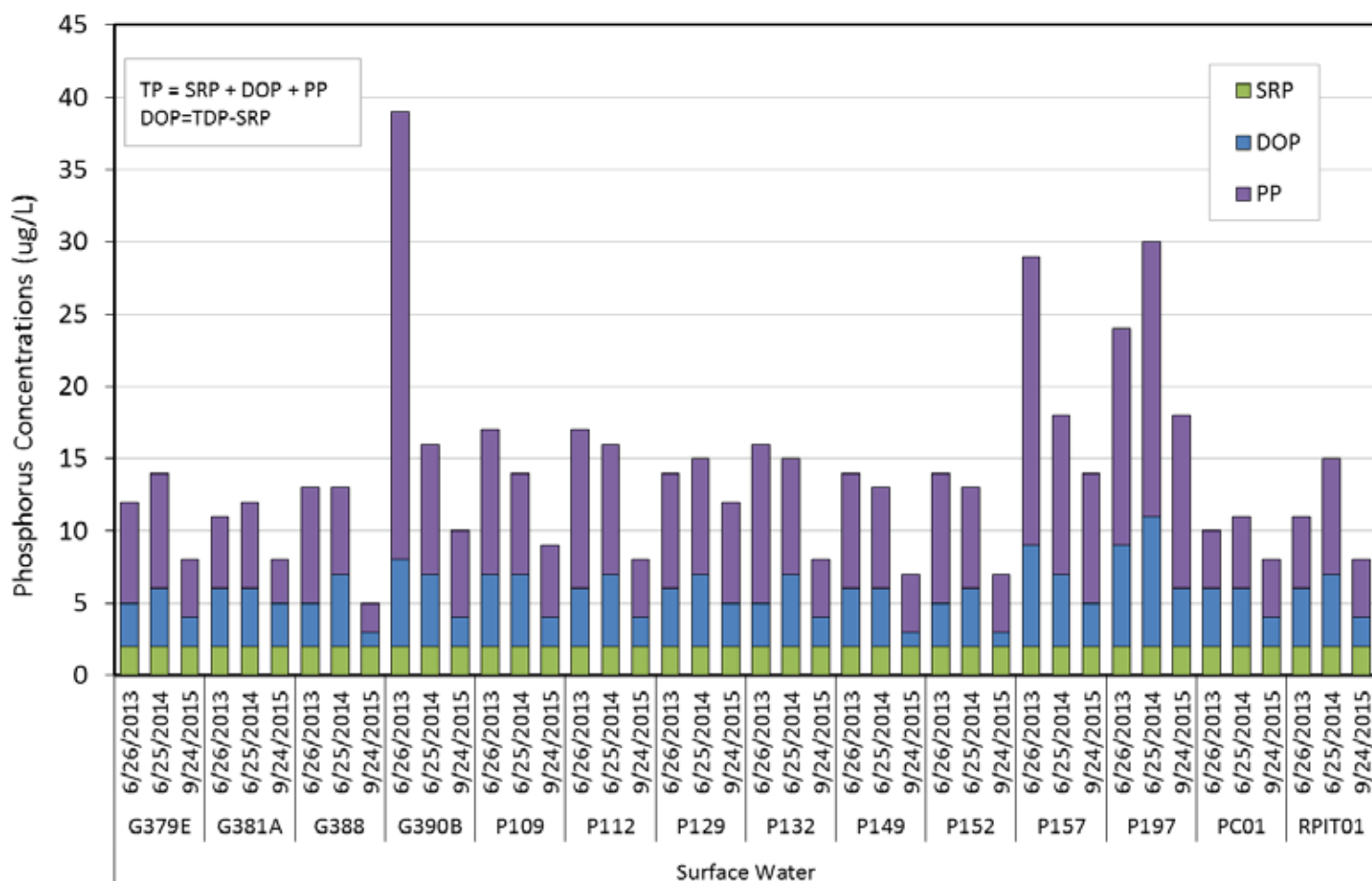
Figure 20. TDP and PP concentrations in surface water samples collected from sites within the PSTA Cell, LSAV Cell, and STA-3/4 Discharge Canal.
