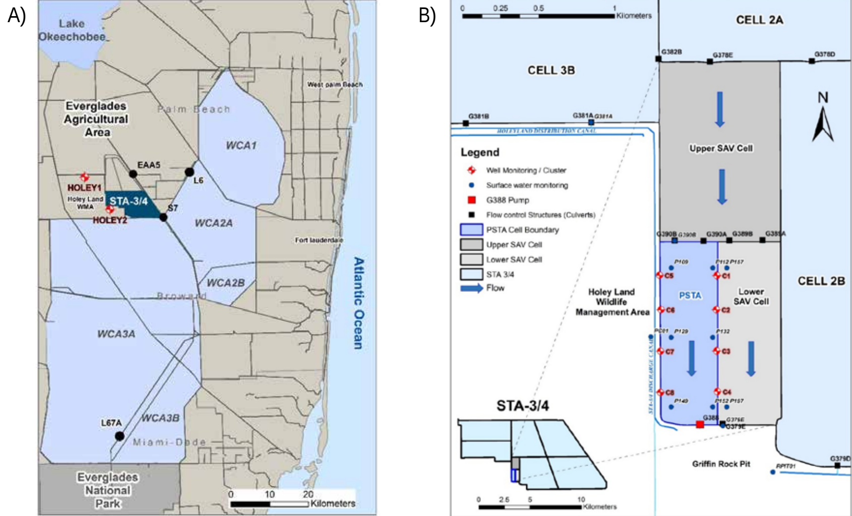
Figure 2. A) Map of the study area showing STA-3/4 and selected rainfall and regional groundwater monitoring stations. B) Map of STA-3/4 showing the PSTA, USAV, and LSAV Cells; related water control structures; monitor well clusters (C1 through C8); and surface water stations. (Note: SAV – Submerged Aquatic Vegetation and WCA – Water Conservation Area.)
