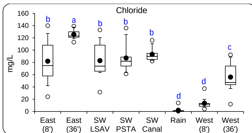
Figure 13. Comparison of Cl concentrations in rainwater, surface water in the LSAV and PSTA cells, and the STA-3/4 Discharge Canal, and groundwater from the shallow (8-ft) and deep (36-ft) wells in milligrams per liter (mg/L) along the PSTA Cell's east and west levees.
