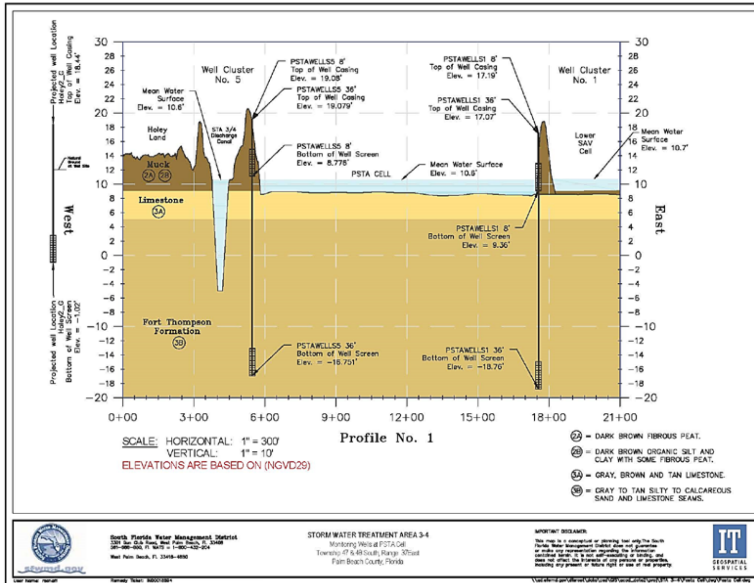
Figure A-2. West to east hydrogeologic cross-section profile through monitor well clusters C5 and C1 illustrating surficial aquifer formations underlying the Holey Land WMA, STA-3/4 Discharge Canal, PSTA Cell, and LSTA Cell.
