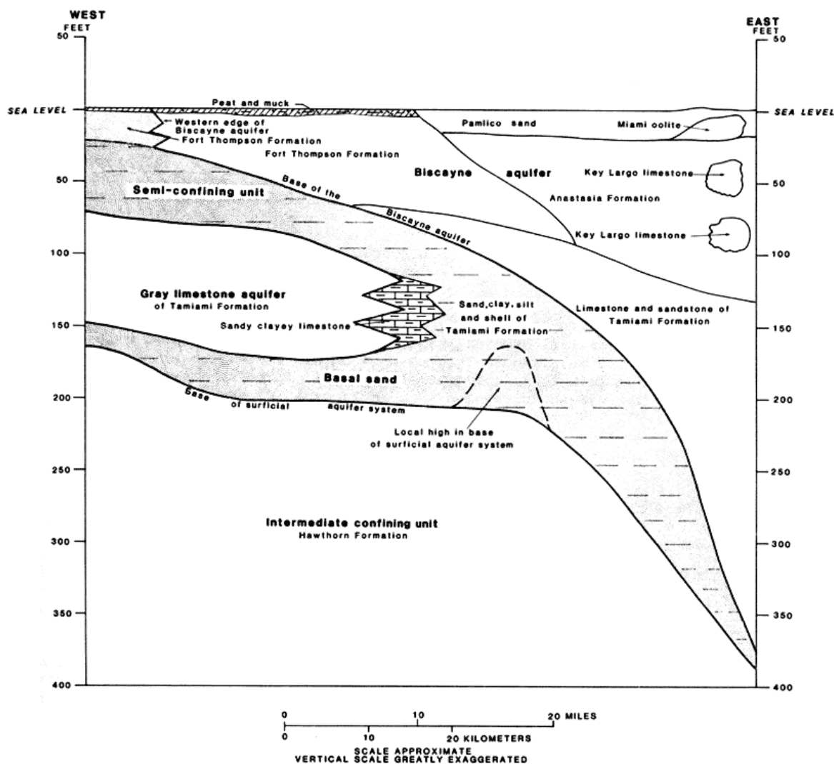
Figure 1. Schematic of geologic formations, aquifers and confining units of the surficial aquifer across Broward County and southwest Palm Beach County near the county line (Fish 1988).
