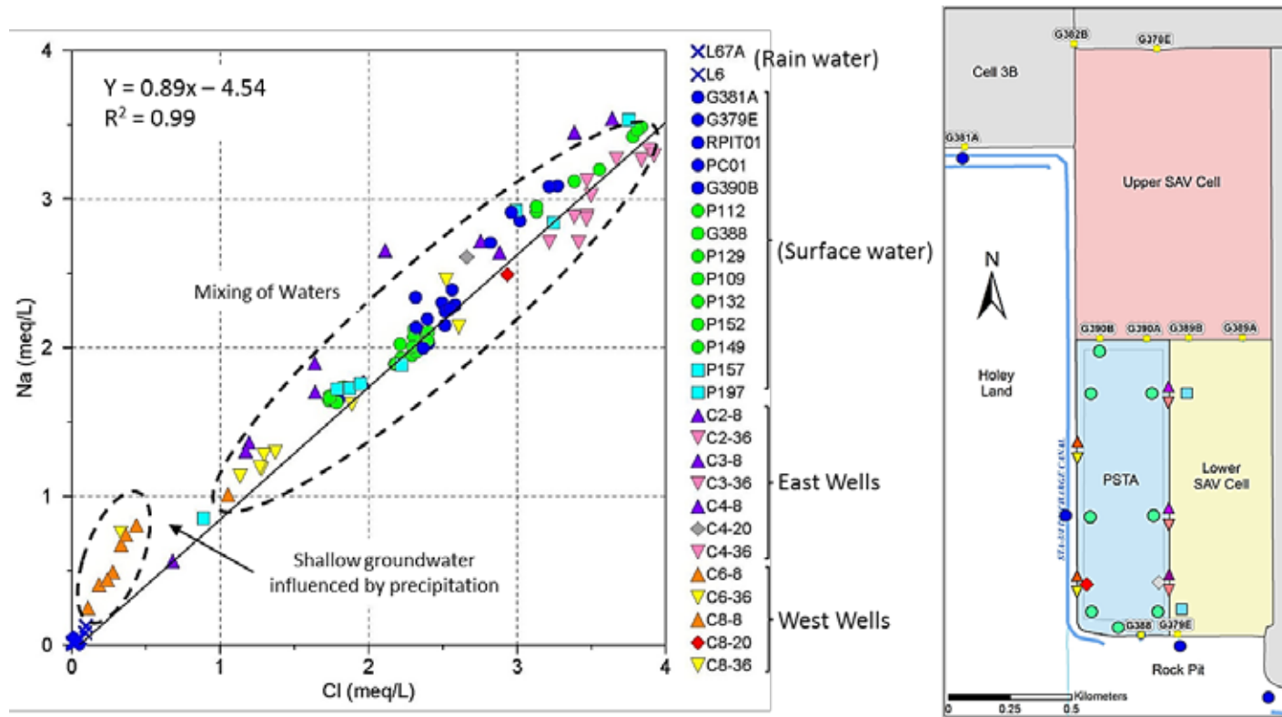
Figure 12. Scatterplot of Na and Cl concentrations in water quality samples in milliequivalents of solute per liter of solvent (meq/L) collected from surface water in the PSTA Cell, groundwater in the shallow (8-ft), intermediate (20-ft), and deep (36-ft) wells located along the PSTA Cell's east and west levees, and rainwater at stations L6 and L67A (see Figure 2 ).
