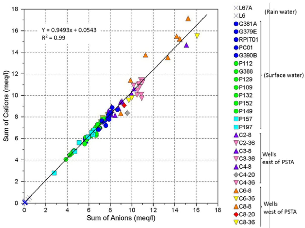
Figure 22. Scatterplots of cation and anion concentrations of rainwater, surface water collected from the PSTA Cell and water control structures, and groundwater from the wells along the PSTA Cell's perimeter levees.
