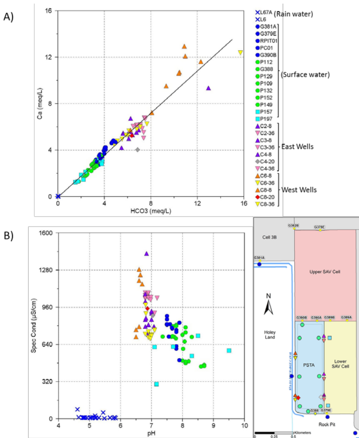
Figure 14. Scatterplots of (A) Ca and HCO 3 concentrations, and (B) specific conductance (Spec Cond) and pH in water quality samples collected from surface water in the PSTA Cell, groundwater in the shallow (8-ft), intermediate (20-ft), and deep (36-ft) wells along the PSTA Cell's east and west levees, and rainwater at stations L6 and L67A (see Figure 2 ).
