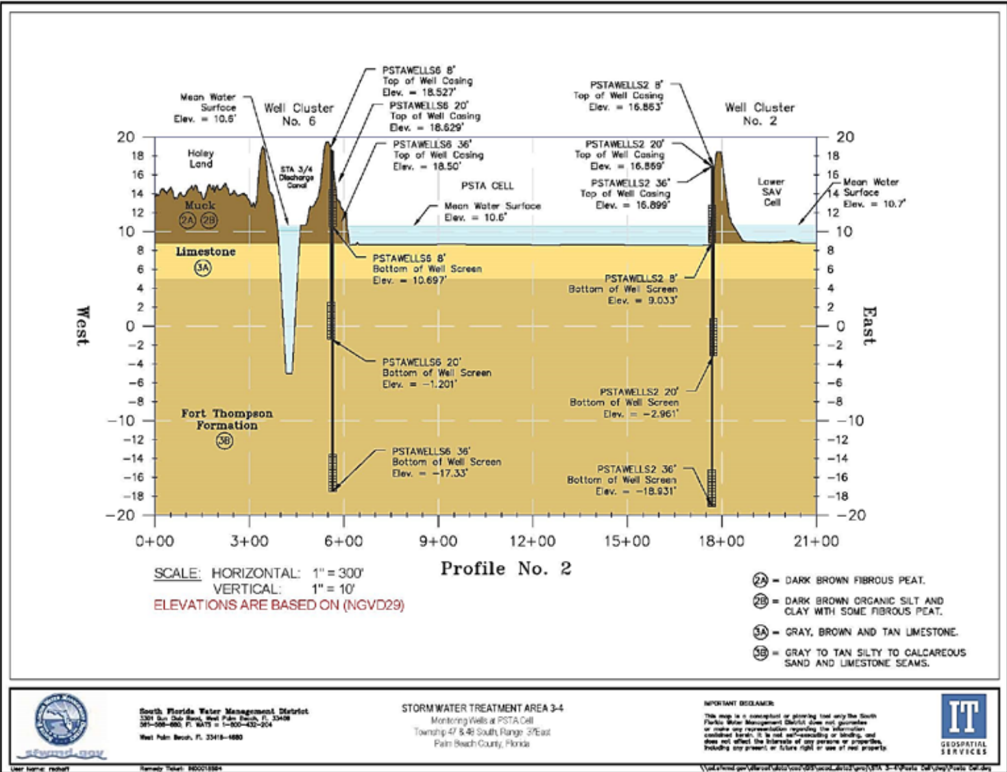
Figure A-3. West to east hydrogeologic cross-section profile through monitor well clusters C6 and C2 illustrating surficial aquifer formations underlying the Holey Land WMA, STA-3/4 Discharge Canal, PSTA Cell, and LSAV Cell.
