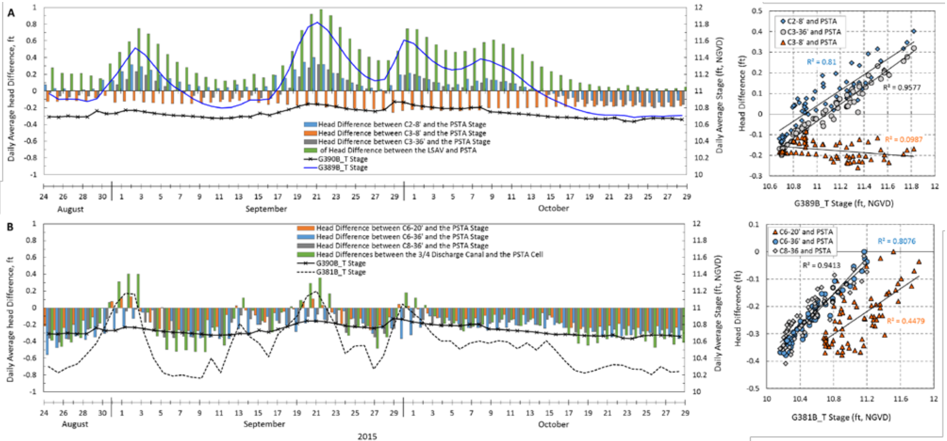
Figure 11. Daily average differences between stages in the PSTA Cell and the groundwater elevations in (A) the PSTA Cell's east levee wells (C2-8', C3-8', and C3-36') and (B) the PSTA Cell's west levee wells (C6-20', C6-36', and C8-36'). Negative head differences indicate that groundwater elevations in the wells were lower than the PSTA Cell stage, while positive head differences indicate that groundwater elevations in the wells were higher than the PSTA Cell stage. Scatterplots show the effect of stages in the LSAV Cell (G389_T) and STA-3/4 Discharge canal (G381B_T) on head differences between perimeter wells and the PSTA Cell.
