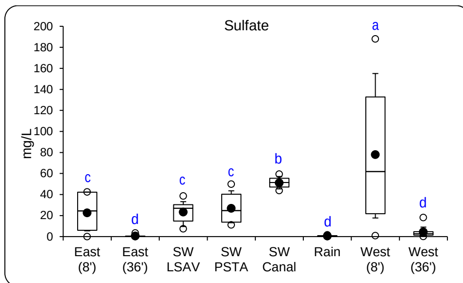
Figure 16. Comparison of SO 4 concentrations in rainwater, surface water in the LSAV and PSTA cells, and groundwater from shallow (8-ft) and deep (36-ft) wells along the PSTA's Cell east and west levees.
