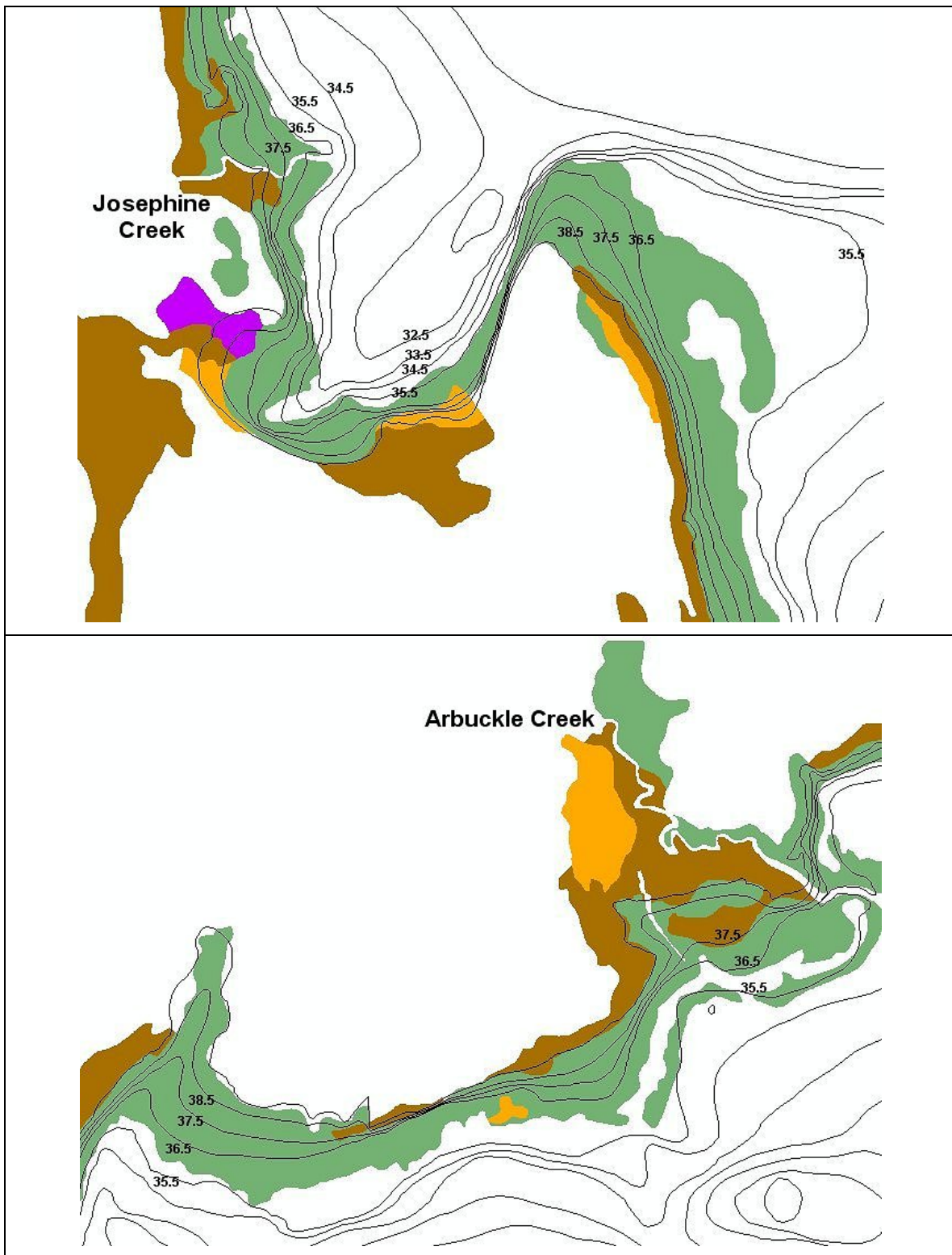
Figure 30. Elevations within Lake Istokpoga Littoral Wetlands at Josephine and Arbuckle Creeks (green areas indicate marsh, brown areas indicate swamp, orange areas indicate shrub and purple areas indicate wet prairie habitats).
