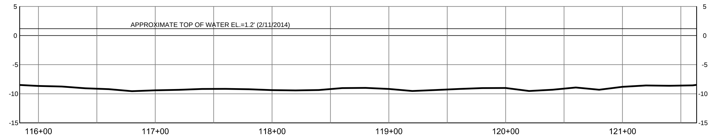
SURVEY BASELINE 'A' PROFILE (Intended Horizontal Display Scale: 1"=50') (Intended Vertical Display Scale: 1"=5')
